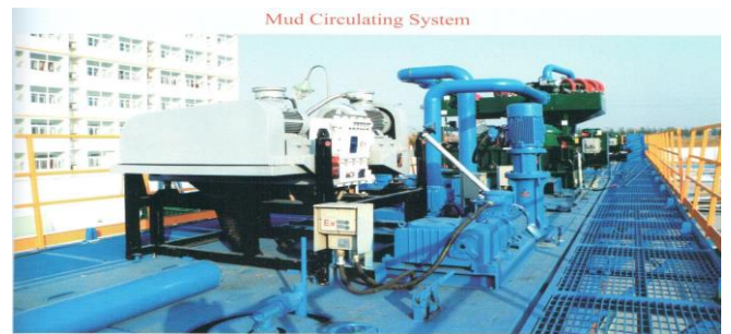
Mud Circulating System
